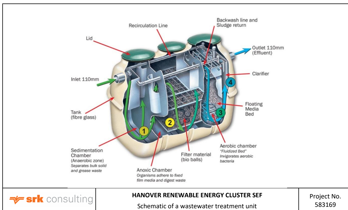
Figure 2-26: Schematic of a wastewater treatment unit
