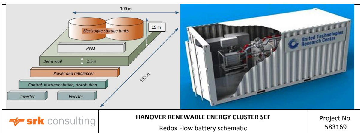
Figure 2-24: Redox Flow battery schematic
