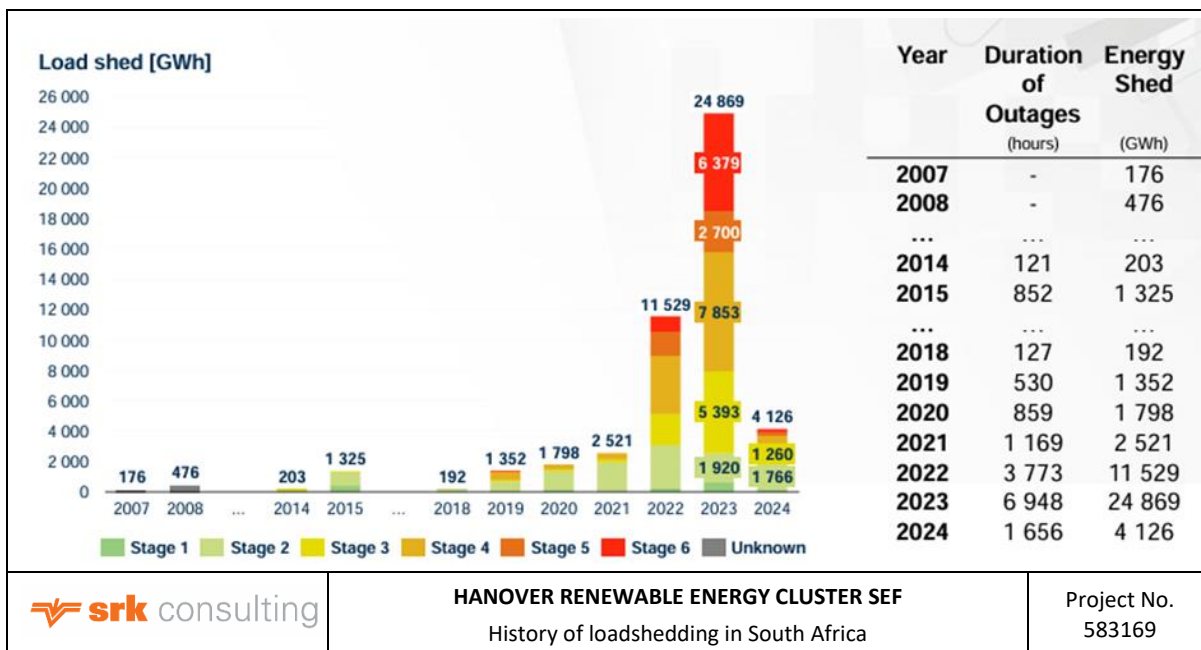
Figure 2-11: History of loadshedding in South Africa
