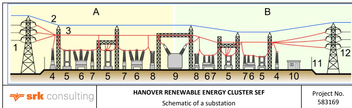
Figure 2-21: Schematic of a substation
