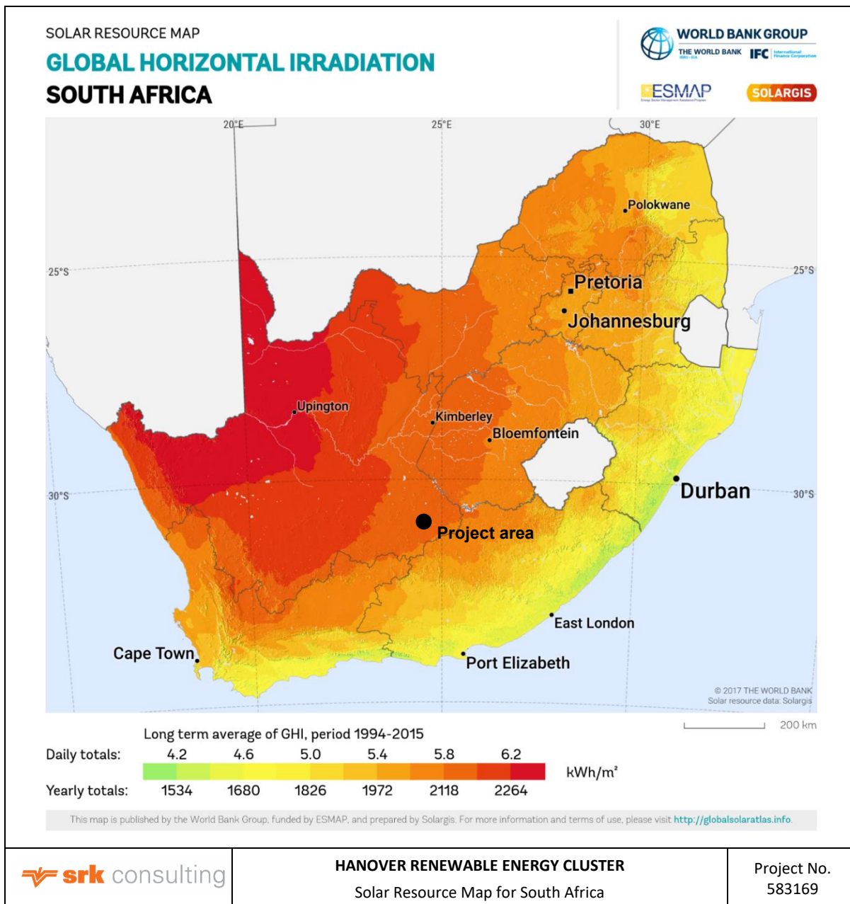
Figure 2-4: Solar resource map for South Africa
