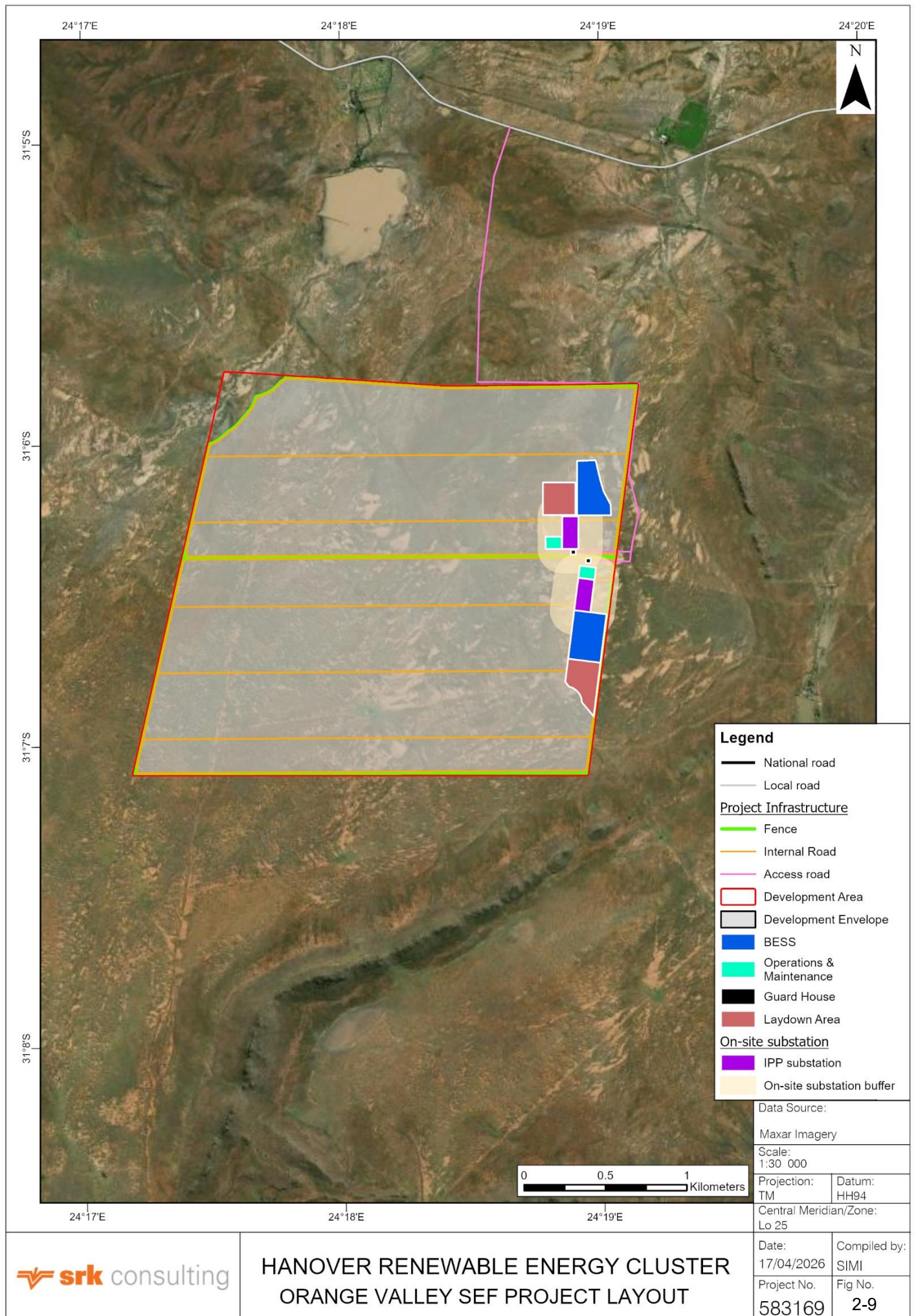
Figure 2-9: Orange Valley SEF project site
