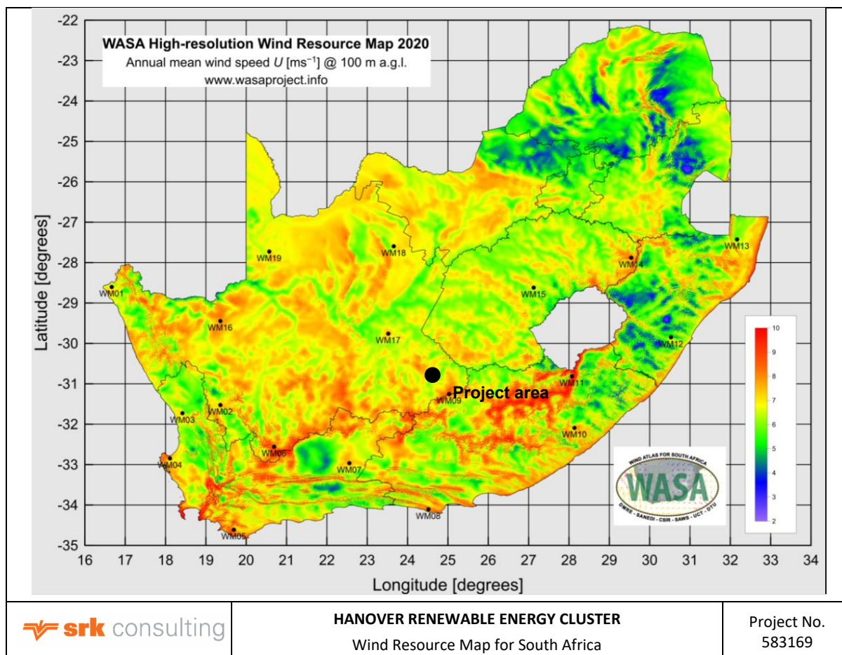
Figure 2-5: Wind resource map for South Africa
